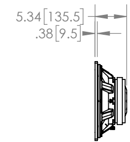
SPEAKER ASSEMBLY SIDE VIEW
